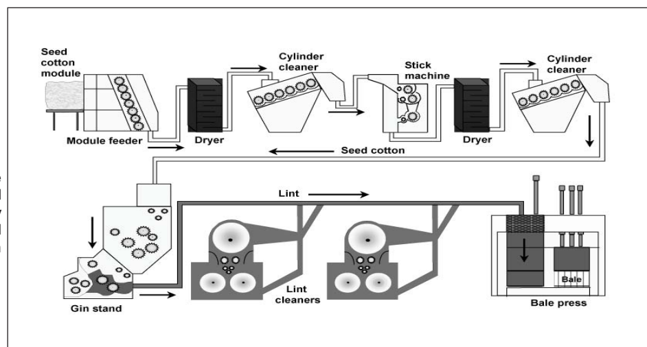
Figure 2.6: Representative cross-sections of typical types of gin machinery arrayed in a sequence used for spindle-picked cotton
