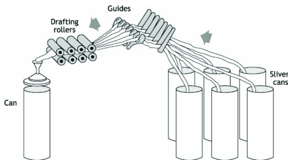
Figure 2.33: Diagram of drawing sliver
